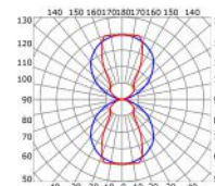
Transparent cover (light reduction: -33%)
