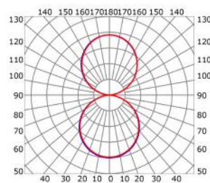
— C0-C180 — C90-C270 Transparent cover (light reduction -26%)
