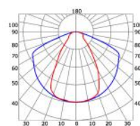
60° lens cover (light reduction: -3%)
