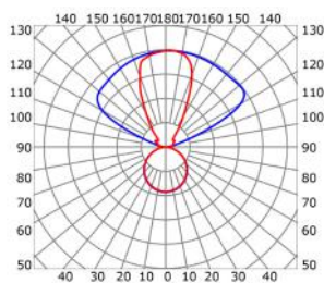
— C0-C180 — C90-C270 Lens 54° cover (light reduction -28%)
