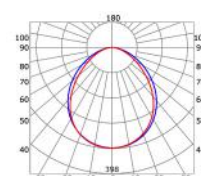
Semiopal cover (light reduction: -9%)
