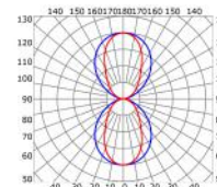
Semiopal cover (light reduction: -36%)
