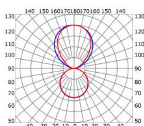
— C0-C180 — C90-C270 Semiopal cover (light reduction -31%)
