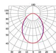
Black diffuser (light reduction: -86%)
